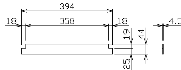
FB4.5X44 (ズレ止め) 詳細
