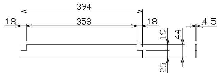
FB4.5X44 (ズレ止め) 詳細
