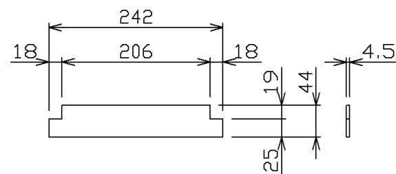
FB4.5X44 (スレ止め) 詳細
